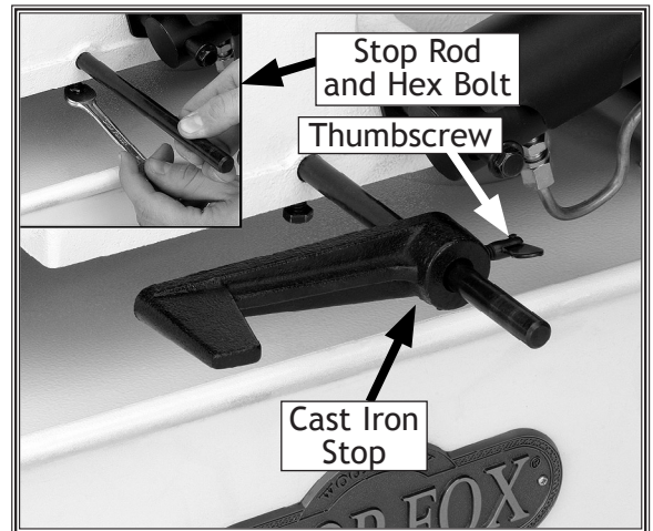
Figure 17. Installing the cast iron stop.
